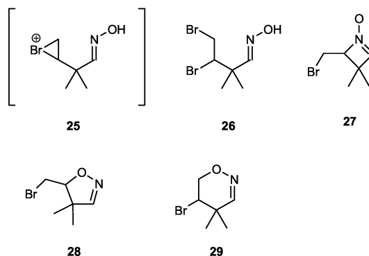
Scheme 9. Bromocyclization of 2,2-dimethyl-3-butene aldioxime; possible intermediates and products.
