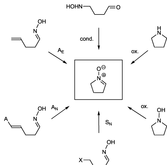
Scheme 1. Principal routes to cyclic nitrones (pyrroline N-oxides).
