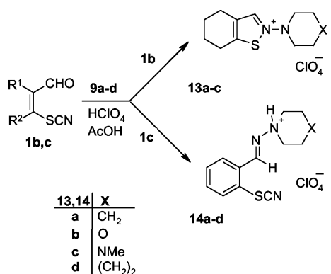
Scheme 2. The reaction of cyclic \beta -thiocyanatovinyl aldehydes with N -amino heterocycles.
