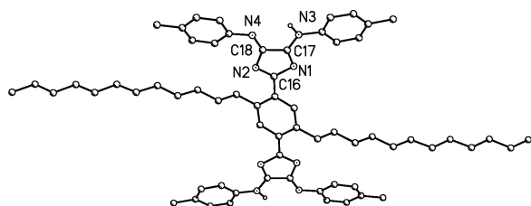
Fig. 2. Molecular structure of bis-4 H -imidazole 3j in the solid state. Selected bond lengths [Å]: C16–N2 1.322(2), C16–N1 1.415(2), C17–N1 1.306(2), C18–N2 1.387(2), C17–C18 1.495(3), C17–N3 1.335(3), C18–N4 1.288(3).
