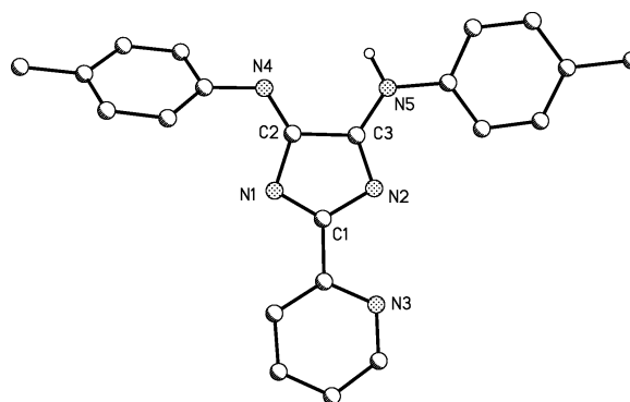
Fig. 1. Molecular structure of 4 H -imidazole 3a in the solid state. Selected bond lengths [Å]: C1–N2 1.403(5), C1–N1 1.311(5), C3–N2 1.314(5), C2–N1 1.407(5), C2–C3 1.506(5), C2–N4 1.276(5), C3–N5 1.337(5).
