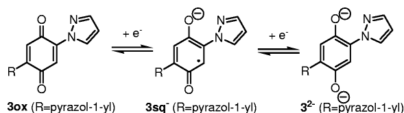
Scheme 5. Reduction of the quinone 3ox .
