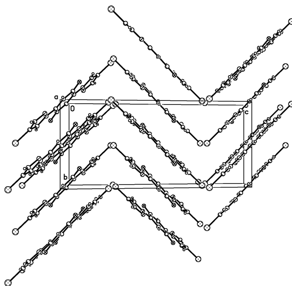
Fig. 16. Packing of the 7ox molecules in the unit cell.
