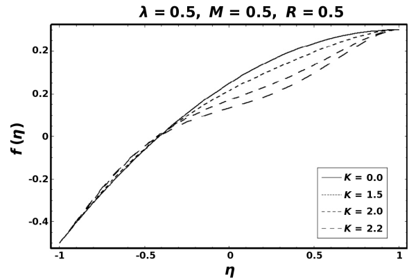
Fig. 13. Influence of K on f when \bar{h} = -0.9 .
