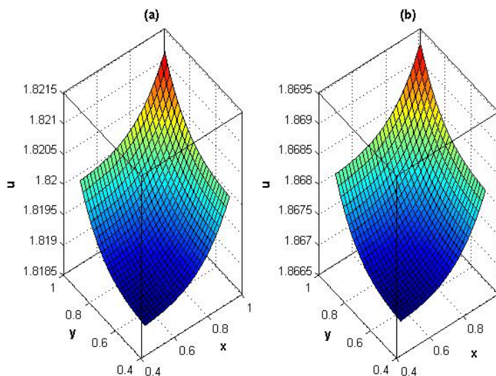
Fig. 4. The surface of the exact and the approximate solutions of (48). (a) The exact solution. (b) The approximate solution obtained in this work.
