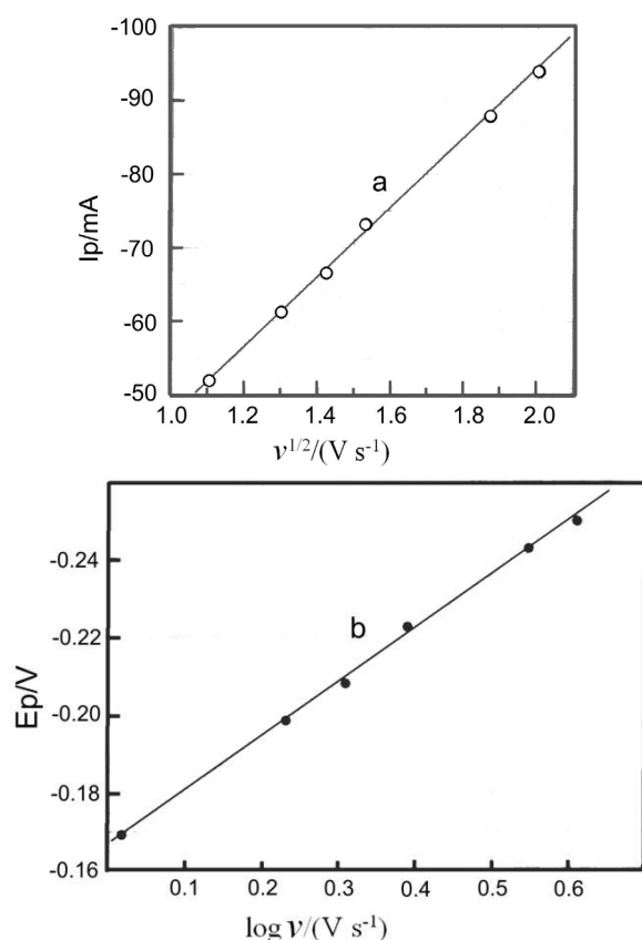
Fig. 4. Dependencies of peak currents (a) and peak potentials (b) of the redox reaction (1) on the sweep rate v > 1.0 V s^{-1} . Area: 0.308 cm^2 ; temperature: 973 K; concentration: 2.64 \cdot 10^{-4} mol cm^{-3} ; reference electrode: Ag/NaCl-KCl-AgCl (2 wt%).
