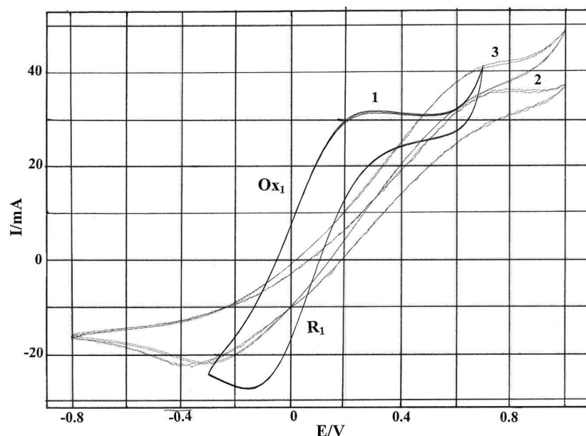
Fig. 2. Cyclic voltammograms for the redox reaction \text{Eu(III)} + e^- \leftrightarrow \text{Eu(II)} in NaCl-KCl-NaBr (15 wt%)- \text{EuCl}_3 melt; 1, 973 K; 2, 1023 K; 3, 1073 K. Sweep rate: 1.0 \text{ V s}^{-1} ; concentration of \text{EuCl}_3 : 8.62 \cdot 10^{-5} \text{ mol cm}^{-3} ; reference electrode: Ag/NaCl-KCl-AgCl (2 wt%).
