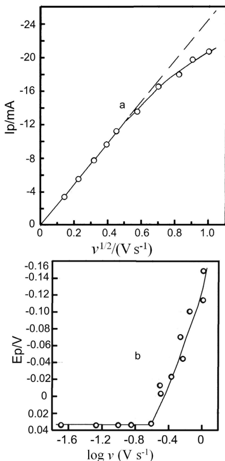
Fig. 3. Dependencies of peak currents (a) and peak potentials (b) of the redox process on the sweep rate. Area: 0.298 cm 2 ; temperature: 973 K; concentration: 8.21 · 10 -5 mol cm -3 ; reference electrode: Ag/NaCl-KCl-AgCl (2 wt%).
