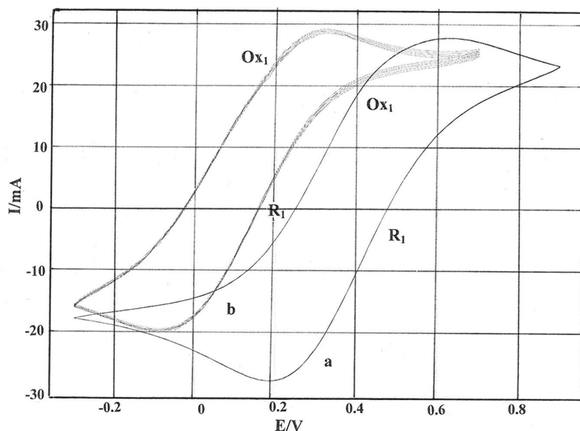
Fig. 1. Cyclic voltammetric curves obtained in NaCl-KCl-EuCl 3 melt: (a) before addition of NaBr; (b) after addition of 5 wt% NaBr. Sweep rate: 1.0 V s -1 ; temperature: 973 K; concentration of EuCl 3 : 6.71 \cdot 10^{-5} mol cm -3 ; reference electrode: Ag/NaCl-KCl-AgCl (2 wt%).
