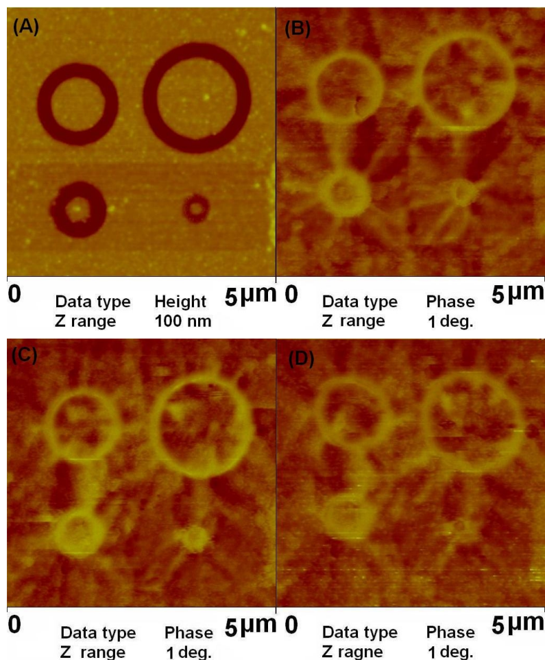
Fig. 7. Atomic and magnetic force micrographs of a GdFeCo thin film electrodeposited on a Pt/Si plate at 70 °C from a mixture of 50:50 mol% \text{ZnCl}_2 -DMSO 2 , 600 mM \text{FeCl}_2 , 200 mM \text{CoCl}_2 , 600 mM \text{GdCl}_3 . Experimental conditions: pulse potential mode; T_{\text{on}}:T_{\text{off}} = 1:5 ; applied deposition potential -0.001 V; Q = 100 mC. (A) AFM; (B) MFM at 0 Oe; (C) MFM at +10 kOe; and (D) MFM at -10 kOe.
