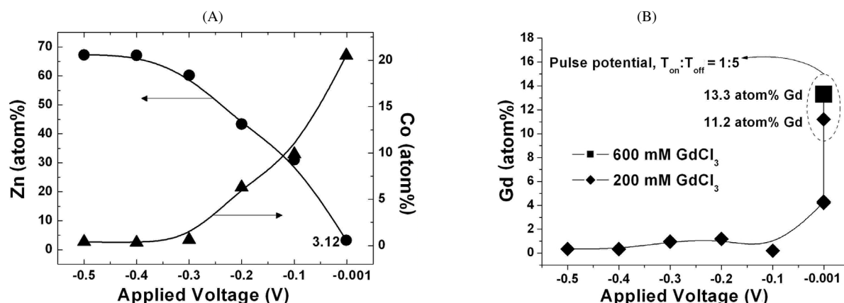
Fig. 2. Relation between layer composition and applied potential for an electrodeposited GdFeCo thin film from 50 : 50 mol% ZnCl 2 -DMSO 2 containing 600 mM FeCl 2 , 200 mM CoCl 2 , 200 mM and 600 mM GdCl 3 at 70 °C. (A) Zn and Co atom%; (B) Gd atom%.
