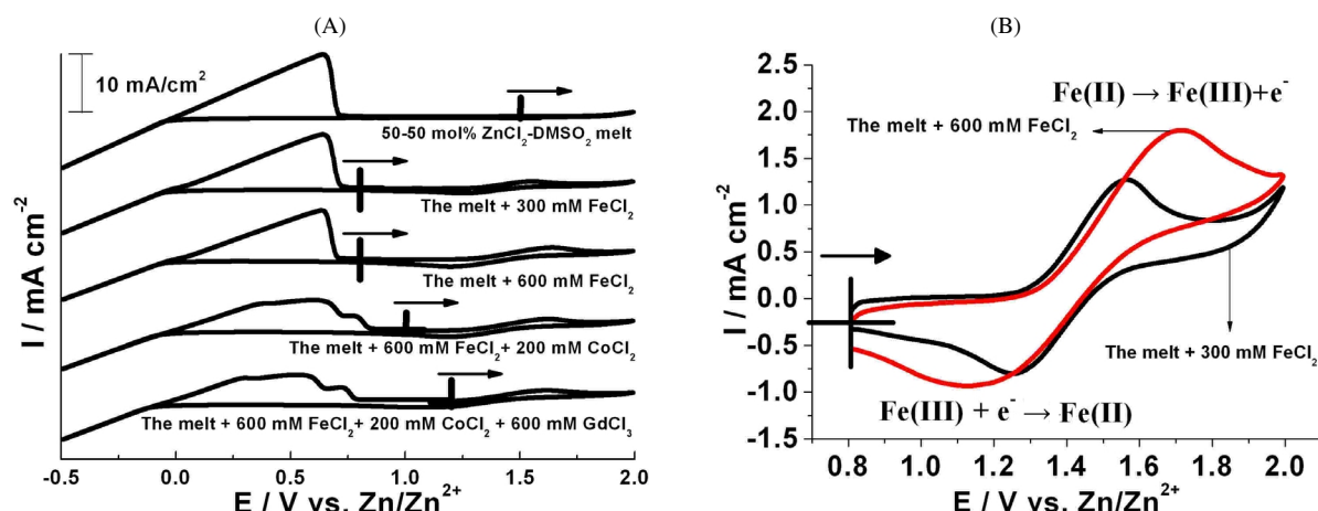
Fig. 1. Cyclic voltammograms recorded on a Pt electrode in 50 : 50 mol% \text{ZnCl}_2 -DMSO 2 containing 300 mM \text{FeCl}_2 , 600 mM \text{FeCl}_2 , 200 mM \text{CoCl}_2 , and 600 mM \text{GdCl}_3 at 70 °C. (A) Overall curve; (B) minor curve for Fe reaction; scan rate: 100 mV/s.
