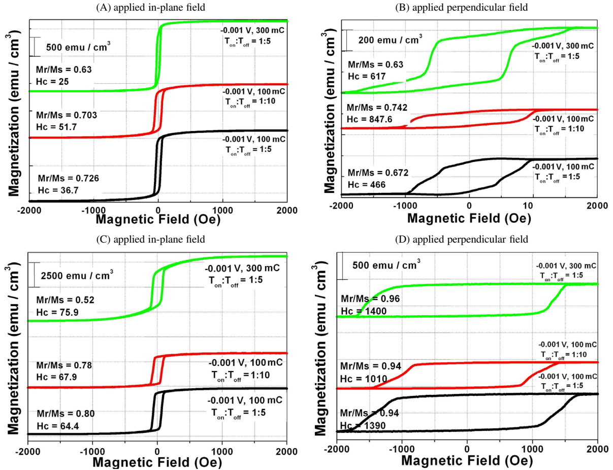
Fig. 4. Hysteresis loops of GdFeCo alloy electrodeposited from a mixture of the 50 : 50 mol% \text{ZnCl}_2 -DMSO 2 , 600 mM \text{FeCl}_2 , 200 mM \text{CoCl}_{2-x}\text{GdCl}_3 melt on a Pt/Si plate at 70 °C. (A), (B) x = 200 mM; (C), (D) x = 600 mM. Experimental conditions: pulse potential mode; T_{\text{on}}:T_{\text{off}} = 1:5 and 1:10 ; applied voltage -0.001 V; Q = 100 and 300 mC.
