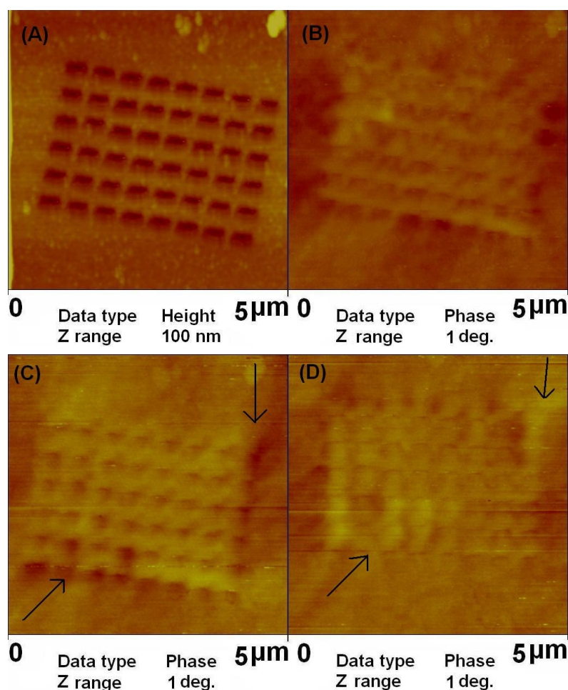
Fig. 8. Atomic and magnetic force micrographs of a GdFeCo thin film electrodeposited on a Pt/Si plate at 70 °C from a mixture of 50:50 mol% \text{ZnCl}_2 -DMSO 2 , 600 mM \text{FeCl}_2 , 200 mM \text{CoCl}_2 , 600 mM \text{GdCl}_3 . Experimental conditions: pulse potential mode; T_{\text{on}}:T_{\text{off}} = 1:5 ; applied deposition potential -0.001 V; Q = 100 mC. (A) AFM; (B) MFM at 0 Oe; (C) MFM at +10 kOe; and (D) MFM at -10 kOe.
