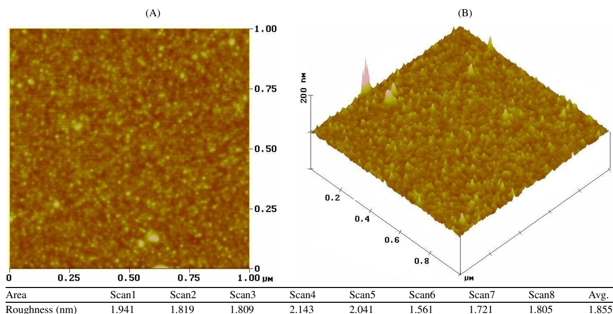
Fig. 6. AFM images of a GdFeCo thin film electrodeposited on a Pt/Si plate at 70 °C from a mixture of 50 : 50 mol% \text{ZnCl}_2 - \text{DMSO}_2 , 600 mM \text{FeCl}_2 , 200 mM \text{CoCl}_2 , 600 mM \text{GdCl}_3 . Experimental conditions: pulse potential mode; T_{\text{on}} : T_{\text{off}} = 1 : 5 ; applied deposition potential -0.001 V; Q = 100 mC. (A) 2-D; (B) 3-D.
