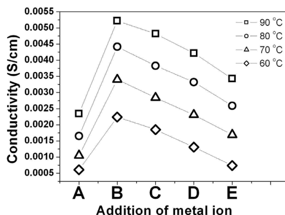
Fig. 3. The isotherms of electrical conductivity as functions of the ionic content in 50 : 50 mol% ZnCl 2 -DMSO 2 at 60–90 °C. A, 50 : 50 mol% ZnCl 2 -DMSO 2 ; B, 50 : 50 mol% ZnCl 2 -DMSO 2 , 600 mM FeCl 2 ; C, 50 : 50 mol% ZnCl 2 -DMSO 2 , 600 mM FeCl 2 , 200 mM CoCl 2 ; D, 50 : 50 mol% ZnCl 2 -DMSO 2 , 600 mM FeCl 2 , 200 mM CoCl 2 , 200 mM GdCl 3 ; E, 50 : 50 mol% ZnCl 2 -DMSO 2 , 600 mM FeCl 2 , 200 mM CoCl 2 , 600 mM GdCl 3 .
