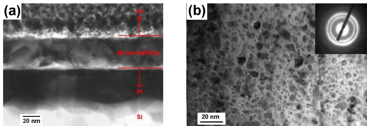
Fig. 5. TEM images of a GdFeCo thin film electrodeposited on a Pt/Si plate at 70 °C from a mixture of 50 : 50 mol% \text{ZnCl}_2 - \text{DMSO}_2 , 600 mM \text{FeCl}_2 , 200 mM \text{CoCl}_2 , 600 mM \text{GdCl}_3 . (a) Section view; (b) plane view. Experimental conditions: applied deposition potential -0.001 V, pulse potential mode; T_{\text{on}} : T_{\text{off}} = 1 : 5 ; Q = 100 mC. The inserted image of a plane view is a diffraction pattern.
