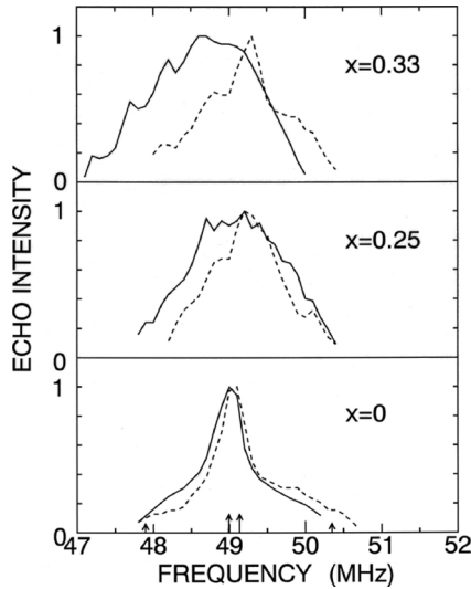
Fig. 1. ^{93}\text{Nb} spectra of \text{Fe}_x\text{NbS}_2 ( x = 0, 0.25, 0.33 ) at 77 K (solid lines) and 300 K (broken lines). They were obtained at t = 80 \mu\text{s} for x = 0 and at t = 52 \mu\text{s} for x = 0.25 and x = 0.33 . The echo intensities are normalized at the peaks. At the bottom, the long arrows indicate the positions of the divergences of the central transition ( -1/2 \leftrightarrow +1/2 ) and the short ones indicate those of the satellite ones ( +1/2 \leftrightarrow +3/2 , -1/2 \leftrightarrow -3/2 ) with values of e^2qQ = 59 \text{ MHz} and K_{\perp} = -0.1\% at 77 K [6] and K_{\parallel} = 0\% .
