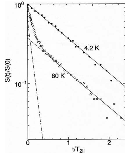
Fig. 2. Decay curve of the ^{93}\text{Nb} spin echo of \text{Fe}_{0.25}\text{NbS}_2 . The broken lines represent the contributions of two components at 80 K. The abscissa is normalized by the respective values of T_{2\text{II}} ( 3220 \mu\text{s} at 4.2 K and 657 \mu\text{s} at 80 K). The value of T_{2\text{I}} at 80 K is 70 \mu\text{s} .
