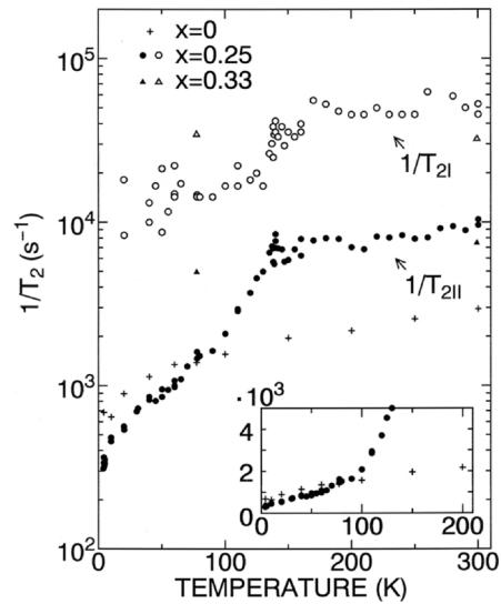
Fig. 3. Temperature dependence of the ^{93}\text{Nb} nuclear spin-spin relaxation rate 1/T_2 of \text{Fe}_x\text{NbS}_2 ( x = 0, 0.25, 0.33 ). For x = 0.25 the values of 1/T_{2I} corresponding to some values of 1/T_{2II} are not shown because of the low accuracy.
