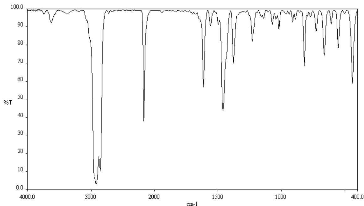
Fig. 1. Infrared spectrum of \text{Ni(4-Chpy)}_2\text{Ni(CN)}_4 in nujol.
