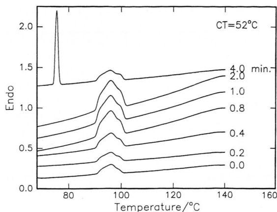
Fig. 5. DSC endotherm profiles of 2-(p- n -heptyloxybenzylidene imino)-5-chloro-pyridine: p - n -octyloxybenzoic acid; (HICP: n OBA) complex at 52°C for different time intervals. CT = crystallization temperature.
