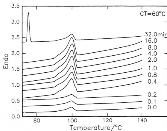
Fig. 6. DSC endotherm profiles of 2-(p- n -heptyloxybenzylidene imino)-5-chloro-pyridine: p - n -octyloxybenzoic acid; (HICP: n OBA) complex at 60°C for different time intervals. CT = crystallization temperature.
