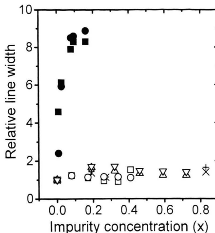
Fig. 4. Relative linewidth of the ^{14}\text{N} NQR line as a function of x in \text{Na}_{1-x}\text{Ag}_x\text{NO}_2 ( \nu_+ : ■, \nu_- : ●), [\text{NaNO}_2]_{1-x}[\text{KNO}_3]_x ( \nu_+ : □, \nu_- : ○), [\text{NaNO}_2]_{1-x}[\text{NaNO}_3]_x ( \nu_+ : △, \nu_- : ▽), and [\text{NaNO}_2]_{1-x}[(\text{CH}_2)_6\text{N}_4]_x ( \nu_+ : +, \nu_- : ×).
