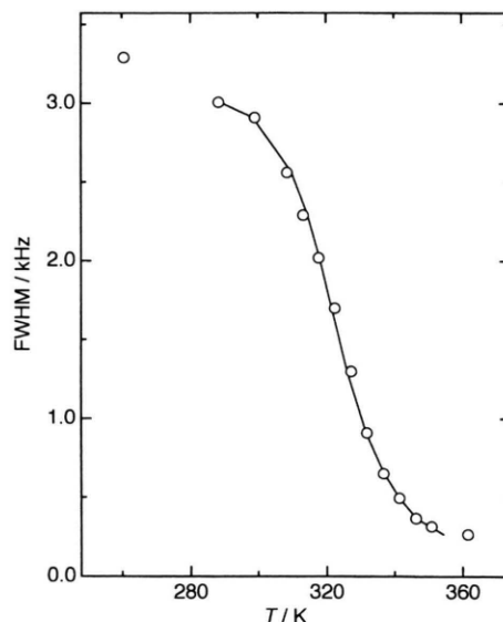
Fig. 14. Temperature dependence of the FWHM of ^{23}\text{Na} NMR for \text{NaInBr}_4 .
