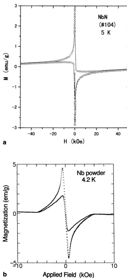
Fig. 4. (a) A hysteresis loop of the magnetization of NbN powder at 5 K synthesized by HTS (see text). (b) A hysteresis of the magnetization of Nb powder at 4.2 K.
