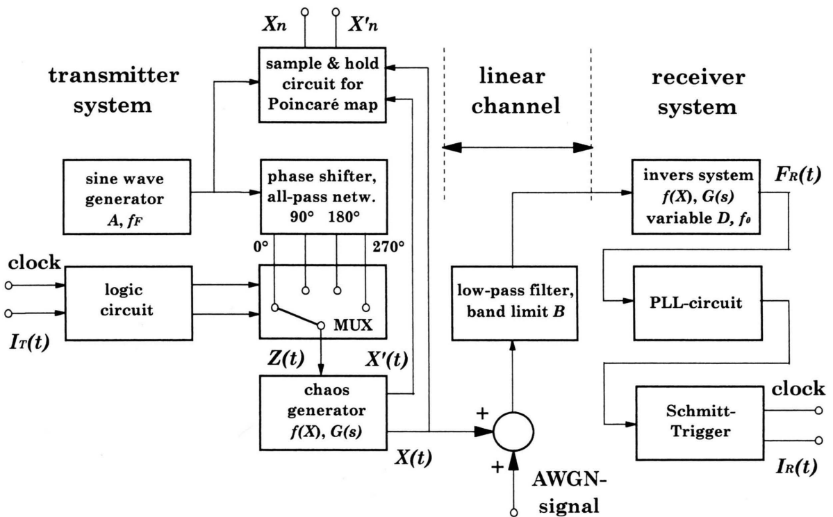
Fig. 4. Block schematic diagram of the communication system.
