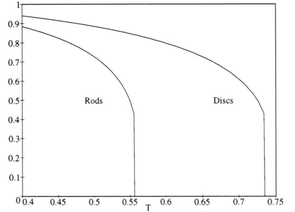
Fig. 2. Temperature dependence of the order parameters \langle P_2 \rangle_A (Rods) and \langle P_2 \rangle_B (Discs) for the unary systems. T denotes the dimensionless temperature.
