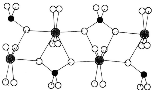
Fig. 4. Chains of edge-connected \text{Eu O}_{6+2} polyhedra [Eu: grey circles; P: full circles; O: open circles]. It is evident how the rare-earth ion links together the \text{PO}_4 chains which run perpendicularly to the drawing plane.
