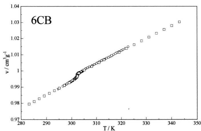
Fig. 2. Specific volumes of 6CB at atmospheric pressure, ( \square this work, \nabla Dunmur et al. [5], \circ Łabno et al. [6]).
