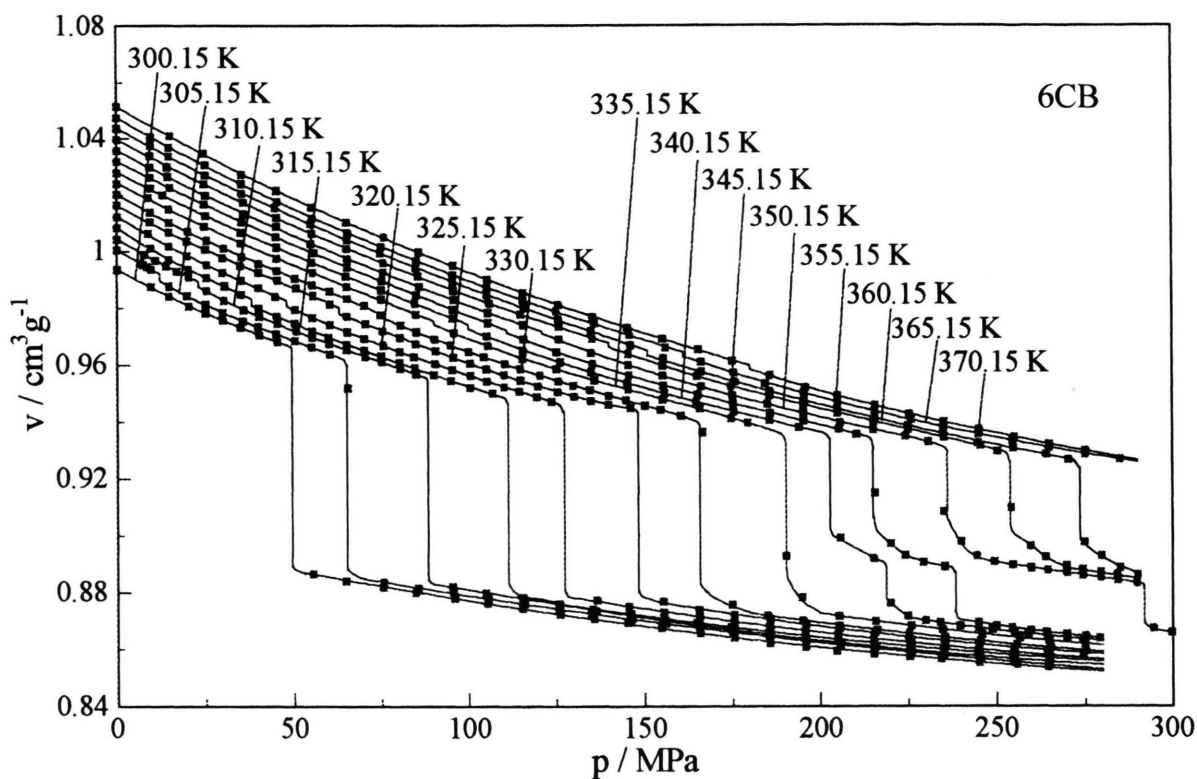
Fig. 1. Specific volumes of 6CB as functions of pressure; the steps in the isotherms refer to the transitions cr_{II} \rightarrow cr_I \rightarrow nematic \rightarrow isotropic . The numerical data can be obtained from the authors.
