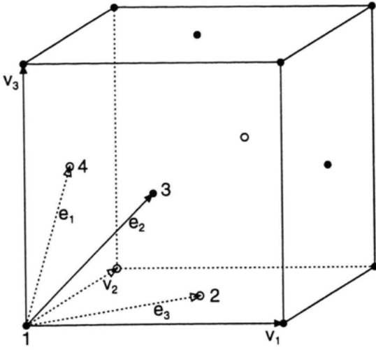
Fig. 2.1. Conventional unit cell of the face centered cubic (FCC) lattice (cf. e.g. [64]) with the primitive translation vectors e_1, e_2, e_3 and the four simple cubic sublattices (the FCC lattice is the infinite periodic extension of the above cell in the directions of v_1, v_2, v_3 ).
