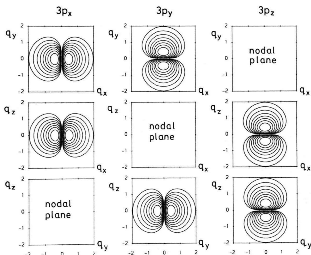
Fig. 10. Schematic momentum-density contour maps of the three degenerate 3p-orbitals of sodium. The measurement probes the momentum density of the 3p y -orbitals along the q_x -axis, the 3p z -orbital being unoccupied.
