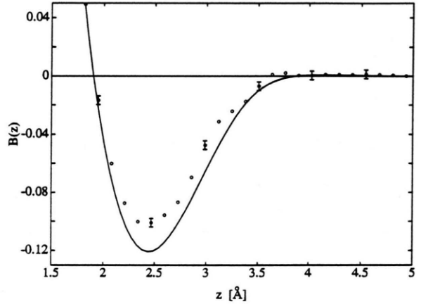
Fig. 2. Experimental and theoretical (solid line) B(z) functions, calculated parallel to the c -axis. The resolution effect is included in the theory. The statistical error is given at some points.
