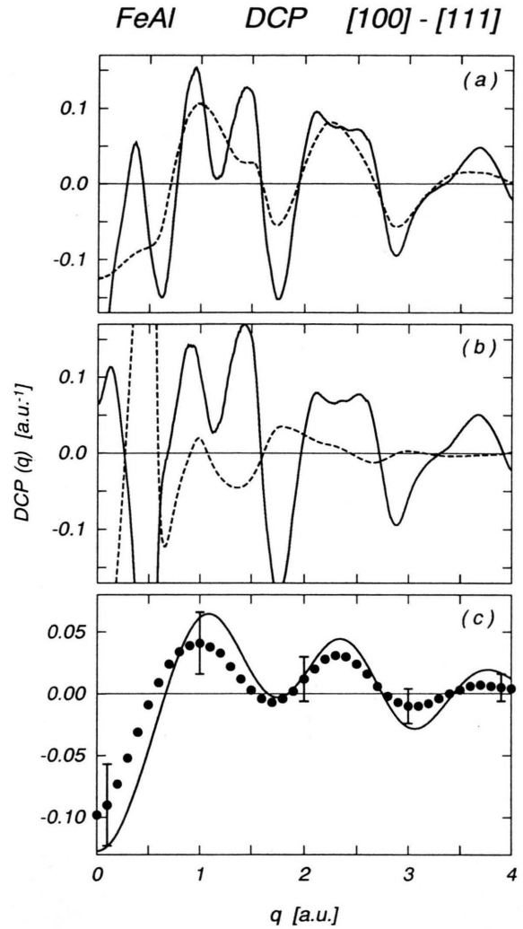
Fig. 4. Compton-profile difference [100]–[111] for FeAl: (a) Calculated unconvoluted differences: Total (solid) and L=4 contribution (dashed). (b) Calculated contributions from the lowest Al s-like band (dashed) and from all other, mainly Fe d-like, bands (solid). (c) Experimental results [24] (bullets) and the present theoretical data convoluted with the experimental residual instrument function (solid).
