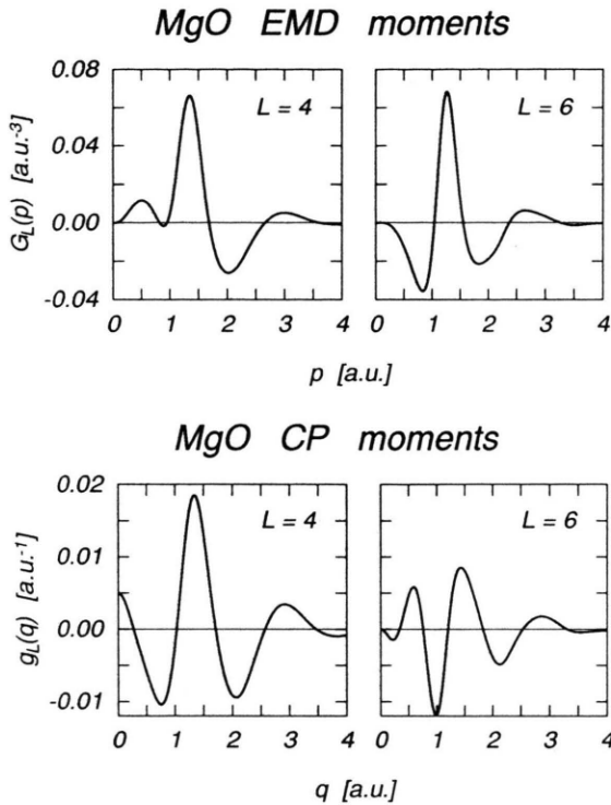
Fig. 1. Expansion coefficients of the electron momentum density (top panel) and of the Compton profile (bottom panel) for MgO.
