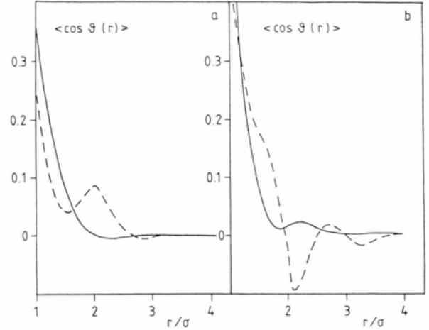
Fig. 6. \langle \cos \theta(r) \rangle dependence on the reverse dipole "temperature". The parameters are as in Figure 5. EXP2 (full line), EXP3 (dashed line).
