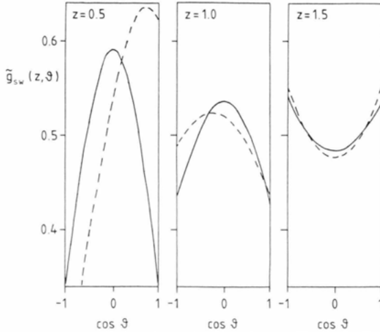
Fig. 9. Normalized orientation density profile \tilde{g}_{sw}(z, \theta) for E^*=0 , c_i=10^{-4} , \mu_s^*=2 (full line) and for E^*=1 , c_i=10^{-1} , \mu_s^*=1 (dashed line). In both cases q_i^*=119 , \eta=0.3665 .
