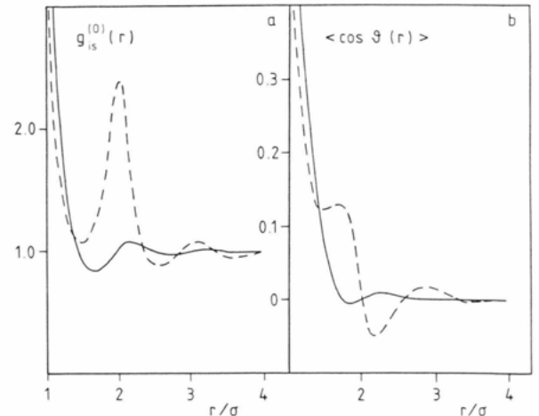
Fig. 7. Angle averaged ion-dipole p.d.f.s (a) and \langle \cos \theta(r) \rangle (b) for c_i = 0.222 , q_i^* = 12 , \mu_s^* = 2 ; EXP2 (full line), EXP3 (dashed line).
