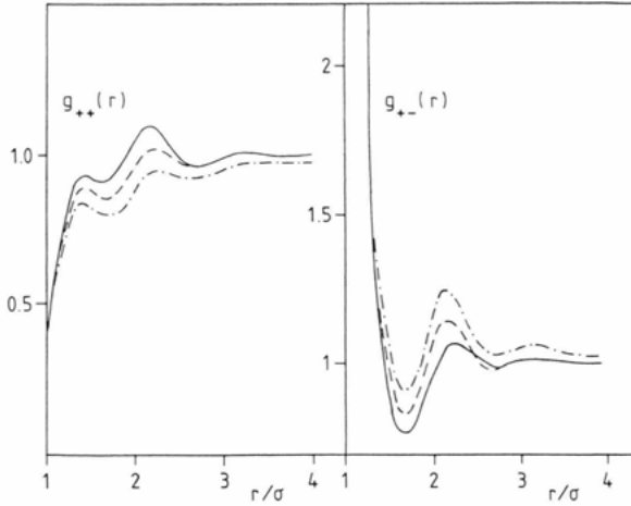
Fig. 4. Concentration dependence of the ion-ion p.d.f.s within EXP2 approximation for q_i^* = 13.6 , \mu_s^* = 3.15 , c_i = 0.5 (full line), c_i = 0.222 (dashed line), c_i = 0.0625 (dash dot).
