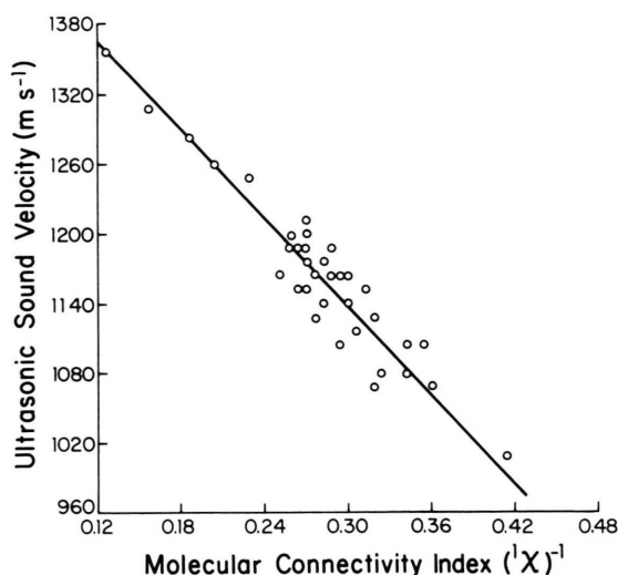
Fig. 1. Plot of the velocity of sound at 20 °C against 1/^1\chi for 35 different alkane molecules.
