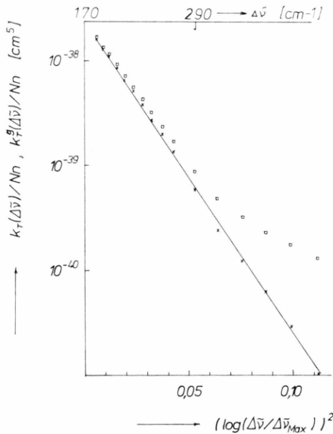
Fig. 13. Blue wing of the outer satellite S_{II} of the Hg-absorption line \lambda 2537 Å, perturbed by Ar; \square\square\square measurement at 513.9^\circ\text{K} ; \times\times\times absorption coefficient k_T^b(\Delta\tilde{\nu})/nN for bound-free transitions.
