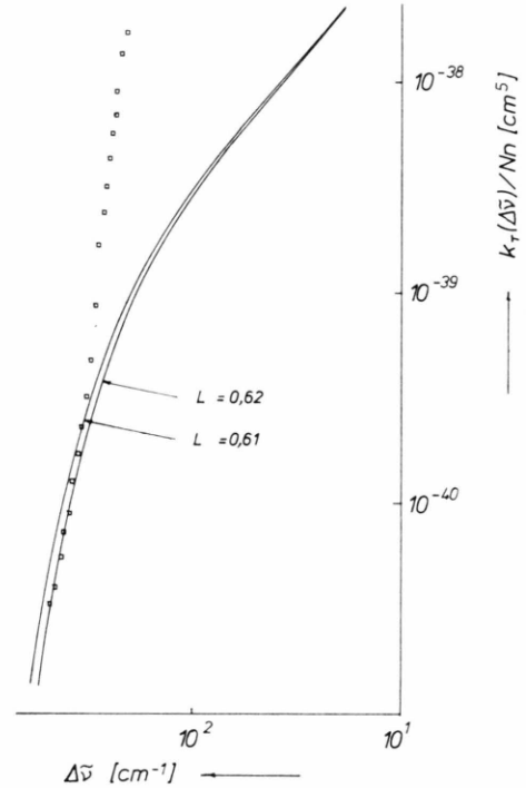
Fig. 14. Blue wing of the Hg-absorption line \lambda 2537 Å, perturbed by Ar. \square\square\square measurement at 513.9^\circ\text{K} ; — theoretical curves k_T^f(\Delta\tilde{\nu}) for C_{6\Sigma} = 0.83 \text{ eV}\text{\AA}^6 .
