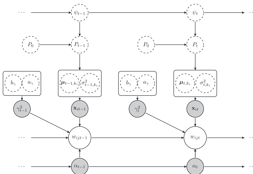
Figure 3: Directed acyclic graph of the proposed dynamic LS model. It exhibits the hierarchical structure of the observations w_{ijt} (solid white circle), the intercept \alpha_t , the latent positions \mathbf{x}_t and variances \gamma_t^2 (gray circles), the parameters of the LS model \mu_{t,k_i} and \sigma_{t,k_i}^2 , the Dirichlet process prior at time t , DP(\psi_t, P_0) , denoted with P_t and its hyper-parameters (dashed white circle). The directed arrows show the causal dependence structure of the model.
