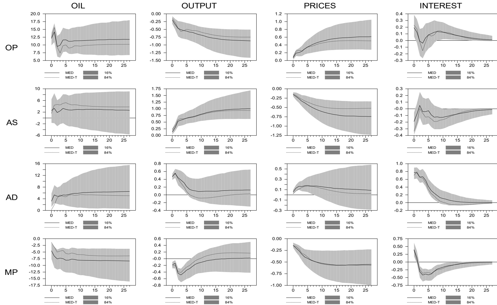
Figure S2: Full sign indentification of Peersman's model by QR. Acceptance rate =0.0313%.
