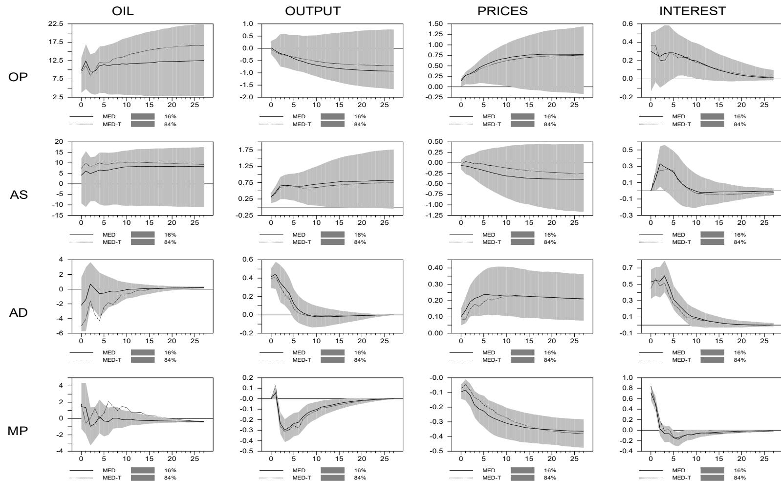
Figure S1: Full parametric identification of Peersman's model.
