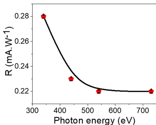
Figure S1: The sensitivity of the fabricated As(III)OI/I-PNMP/PPy optoelectronic device through the evaluation of the wavelengths.
