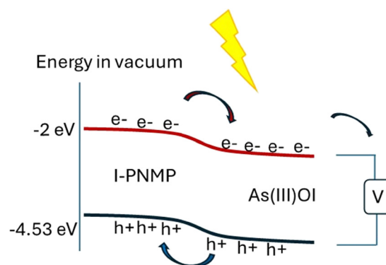
Figure S3: The schematic diagram of the electron transfer through the As(III)OI/I-PNMP/PPy-based device.
