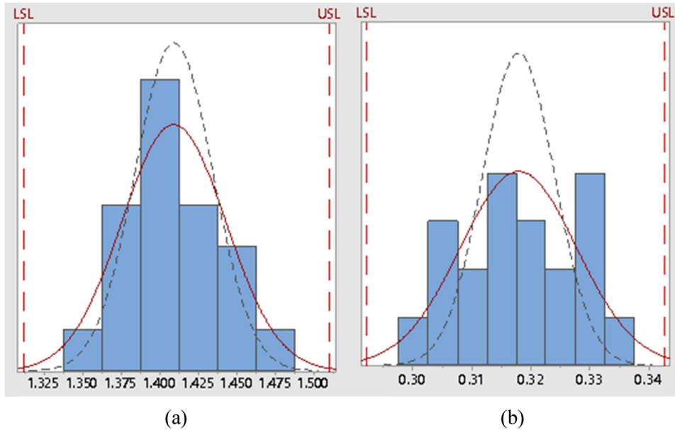
Figure 5: Histograms: (a) surface roughness and (b) circularity.
