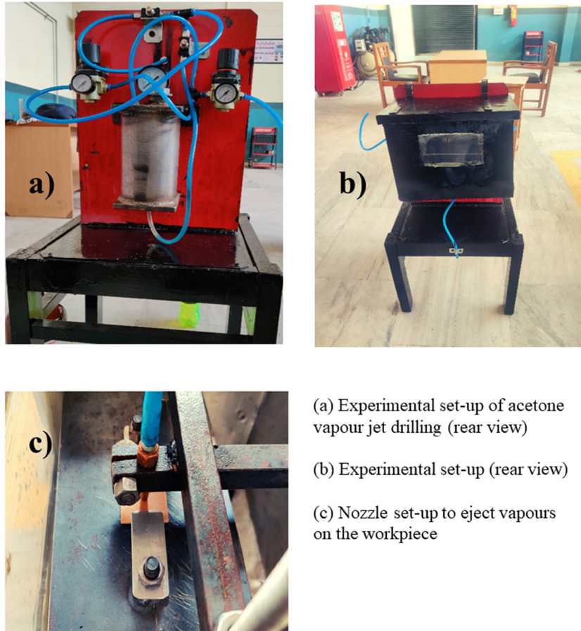
Figure 3: (a–c) Components of the experimental setup.
