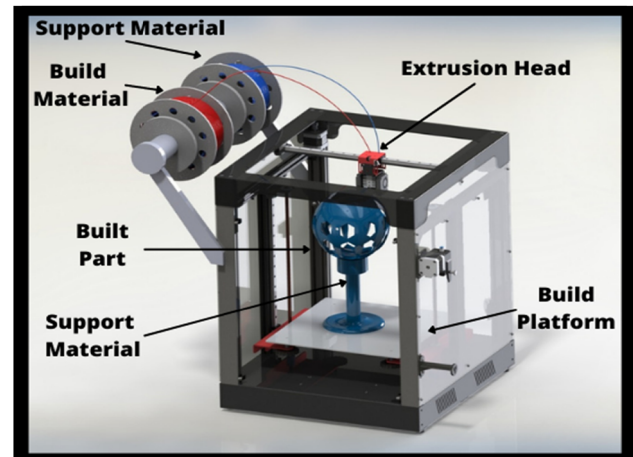
Figure 1: FDM apparatus setup [6].
