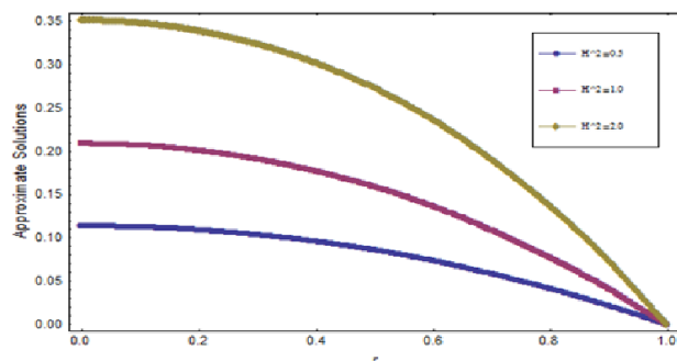
Figure 1: Graph of numerical results for \alpha = 0.5, \gamma = 2, \beta = 1 and several values of H .
