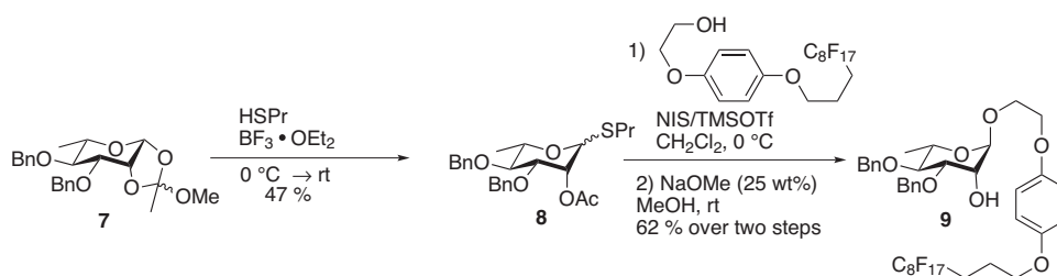
Scheme 2: Acceptor synthesis.
