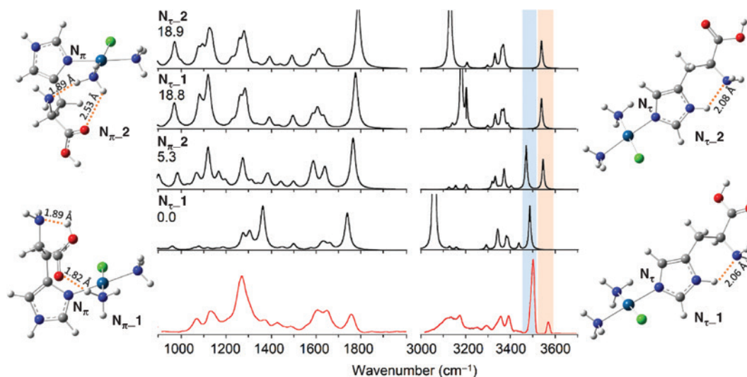
Fig. 6: IRMPD spectrum of cis\text{-[PtCl(NH}_3)_2\text{His}]^+ (red profile) compared to the unscaled linear anharmonic IR spectra calculated at B3LYP/6-311+G(d,p) (Pt=LANL2TZ) level for the most stable conformers of N_\pi and N_\tau families of isomers (black profiles). Optimized geometries at the same level of theory are reported together with relative free energies at 298 K in \text{kJ mol}^{-1} calculated at the \omega\text{B97X-D/6-311+G(d,p)} level.
