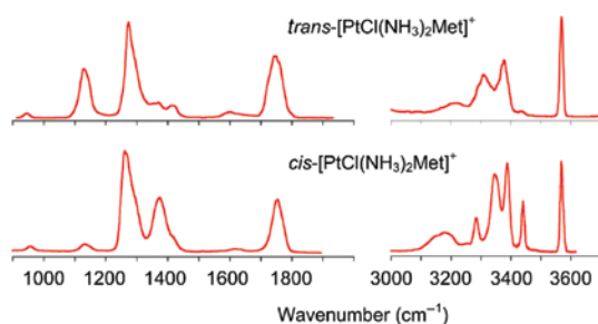
Fig. 8: IRMPD spectra of cis -[PtCl(NH 3 ) 2 Met] + and trans -[PtCl(NH 3 ) 2 Met] + complexes.
