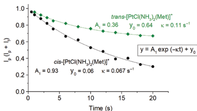
Fig. 11: Plots showing the decay of the relative abundances of the sampled ions, cis - and trans - [\text{PtCl}(\text{NH}_3)_2\text{Met}]^+ , as a function of the irradiation time. Fitting exponential functions are reported.
