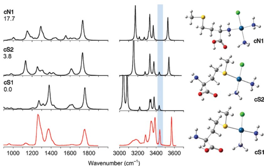
Fig. 9: IRMPD spectrum of cis -[PtCl(NH 3 ) 2 Met] + (red profile), compared with calculated unscaled anharmonic spectra of selected isomers at the B3LYP/6-311++G(2df,pd) level using the 6-311++G(3df) basis set for S and the pseudopotential LANL2TZ-f for Pt. The corresponding optimized geometries are shown on the right. Relative free energies at 298 K in kJ mol -1 are reported.
