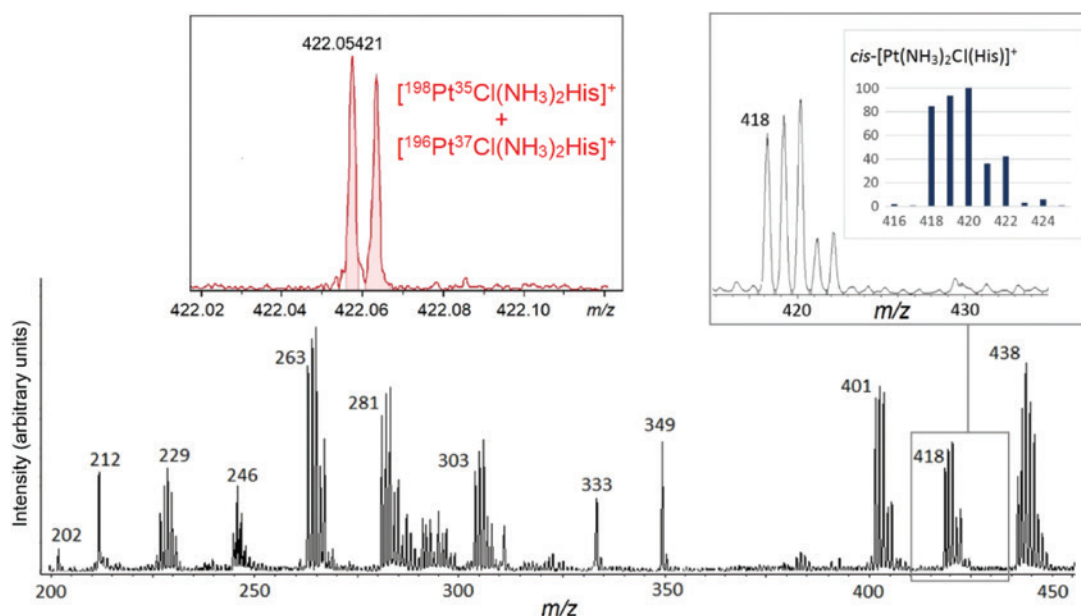
Fig. 5: Mass spectrum of a solution of cisplatin and His (1:1) 5 \times 10^{-5} M in 50:50 methanol/water. The species of interest, the cis\text{-[PtCl(NH}_3)_2\text{His}]^+ complex, corresponds to the cluster at m/z 418. The assignment is consistent with the isotopic pattern enlarged in the inset, matching the calculated distribution (blue sticks) congruent with the presence of one platinum and one chlorine atom. High resolution FT-ICR mass spectra (an excerpt shown on the upper left panel) confirm the elemental composition.
