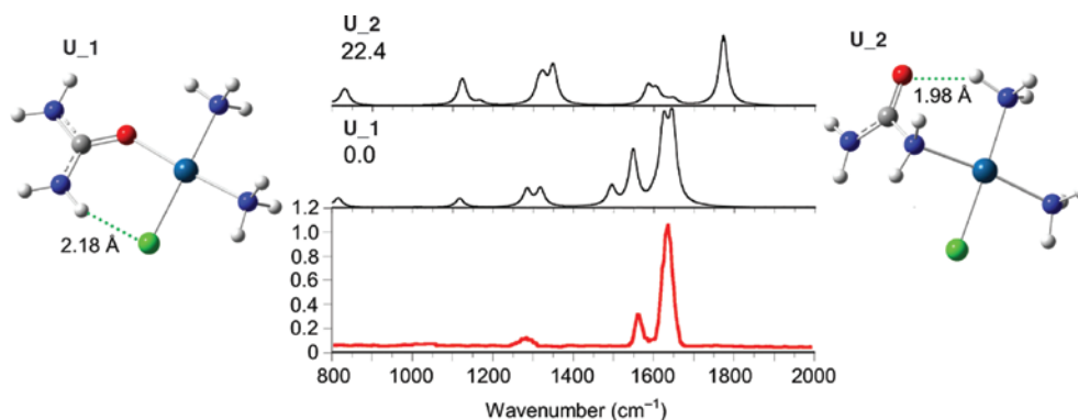
Fig. 3: IRMPD spectrum of cis -[PtCl(NH 3 ) 2 (Urea)] + (red profile) compared with calculated harmonic IR spectra of U_1 and U_2 isomers optimized at the B3LYP/6-311 + G(d,p) (Pt = LANL2TZ) level (black profiles). Relative free energy at 298 K, in kJ mol −1 , is given under each U_1/2 label. Theoretical spectra are scaled by a 0.974 factor.
