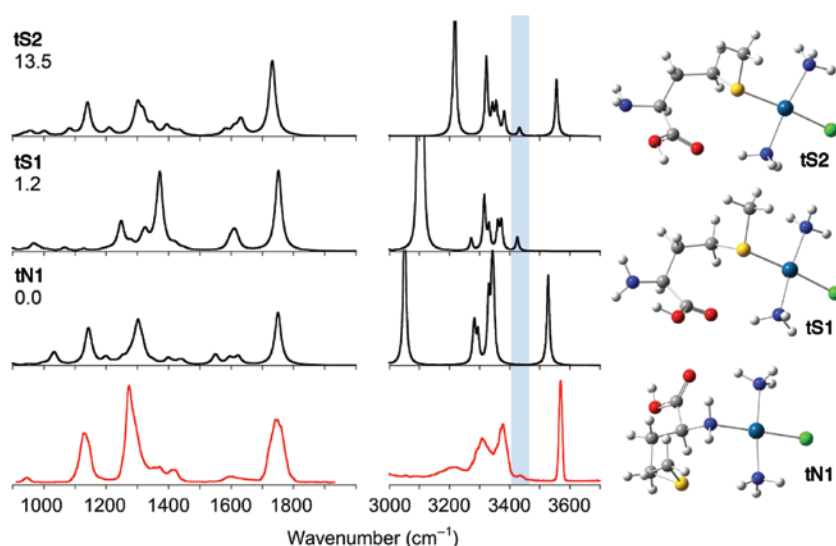
Fig. 10: IRMPD spectrum of trans - [\text{PtCl}(\text{NH}_3)_2\text{Met}]^+ (red profile), compared with calculated unscaled anharmonic spectra of selected isomers at the B3LYP/6-311++G(2df,pd) level using the 6-311++G(3df) basis set for S and the pseudopotential LANL2TZ-f for Pt. The corresponding optimized geometries are shown on the right. Relative free energies at 298 K in \text{kJ mol}^{-1} are reported.
