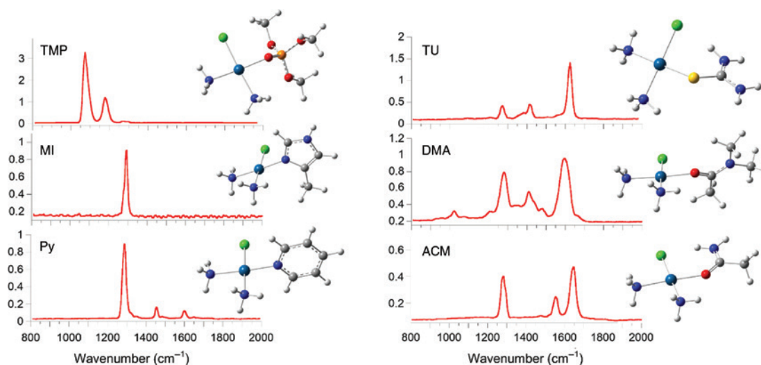
Fig. 4: IRMPD spectra of \text{cis-}[\text{PtCl}(\text{NH}_3)_2(\text{L})]^+ complexes. Also shown are the structures assigned on the basis of the matching between IRMPD spectra and IR spectra of the optimized geometries at B3LYP/6-311+G(d,p) (Pt = Lanl2TZ) level of theory.
