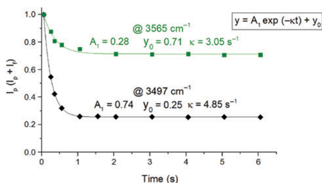
Fig. 7: Plot showing the decay of the parent ion \text{cis-}[\text{PtCl}(\text{NH}_3)_2\text{His}]^+ abundance as a function of irradiation time at two different wavenumbers. Fitting exponential functions are reported.
