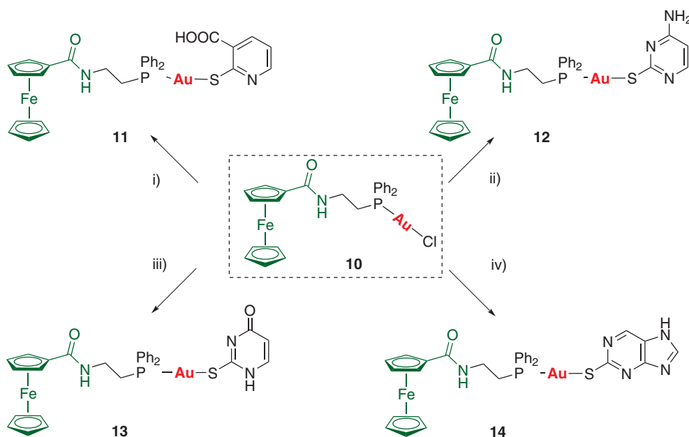
Scheme 1: Synthesis of thiolate gold complexes 11–14 with the ligand \text{PPh}_2\text{CH}_2\text{CH}_2\text{NHCOFc} . (i) 2-mercaptanonic acid + \text{K}_2\text{CO}_3 , (ii) 2-thiocytosine + \text{K}_2\text{CO}_3 , (iii) 2-thiouracil + \text{K}_2\text{CO}_3 , (iv) 2-mercaptapurine + \text{K}_2\text{CO}_3 .
