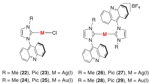
Fig. 4: Ag(I) and Au(I) complexes 22–29 containing acridine-based NHC ligands.
