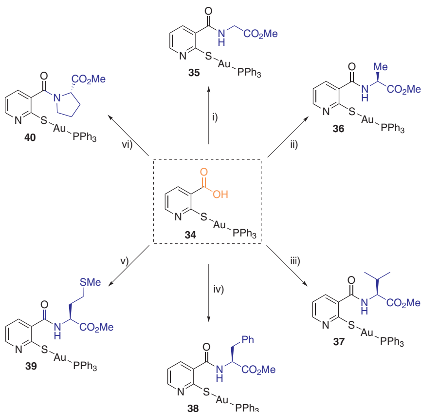
Scheme 4: Synthesis of complexes 35–40 : (i) Glycine methyl ester, DIPEA, PyBOP; (ii) alanine methyl ester, DIPEA, PyBOP; (iii) valine methyl ester, DIPEA, PyBOP; (iv) phenylalanine methyl ester, DIPEA, PyBOP; (v) methionine methyl ester, DIPEA, PyBOP; (vi) proline methyl ester, DIPEA, PyBOP.
