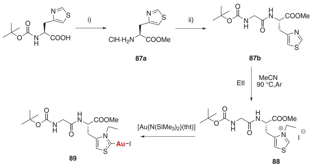
Scheme 8: Synthesis of the thiazolylalanine-containing peptide and the gold carbenes 87–89 . (i) SOCl 2 , MeOH, (ii) Boc-Gly-OH, IBCF, NMM, THF.
