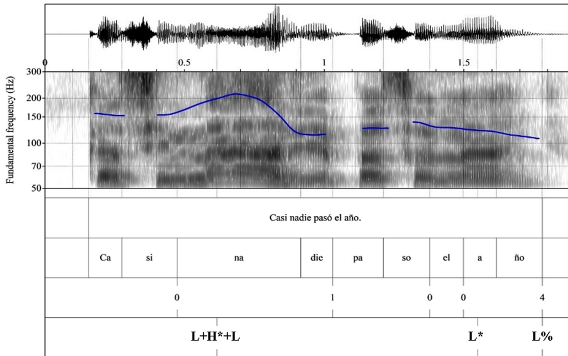
Figure 3: Waveform, spectrogram, and pitch contour for the narrow focus statement ¡Casi na die pasó el año ! “Almost nobody passed the school year!” produced with a tritonal PA (L + H* + L) in prenuclear position and finishing with a low BT.
