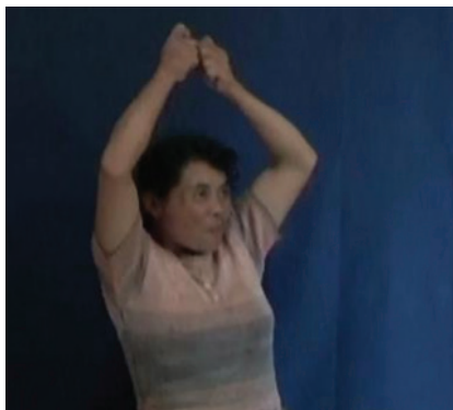
Figure 9. CL_{HL}(SS) -SWING in KK from example (10).
