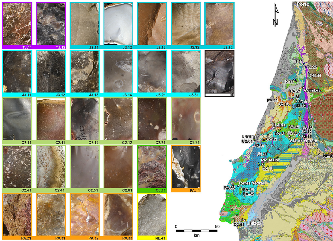
Figure 13: Map of the main flint and siltstone sources from the West Portuguese Meso-Cenozoic Border during Prehistoric times (from Aubry, 2018, p. 16).
