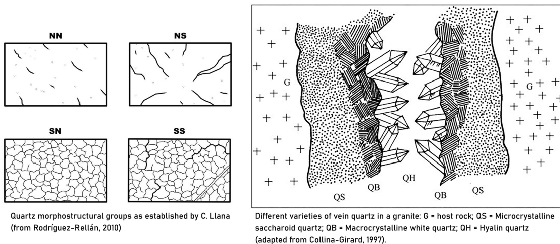
Figure 3: Quartz morphostructural groups.
