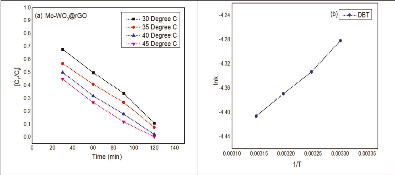
Figure S1: Plot of time vs C_f/C_i (a) and activation energy 1/T vs \ln k (b).
