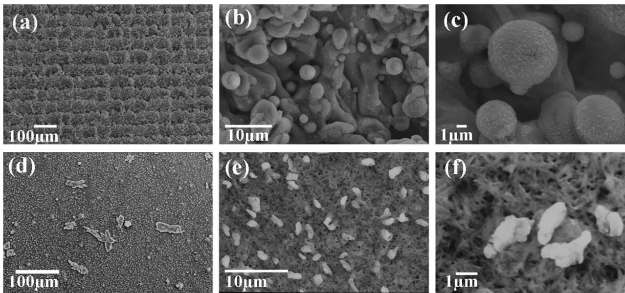
Figure S2: SEM images at different magnification of (a–c) irradiated Ti sample covered with FeCl 3 and without PPy coating and (d–f) PPy coated on Ti surface without laser ablation.
