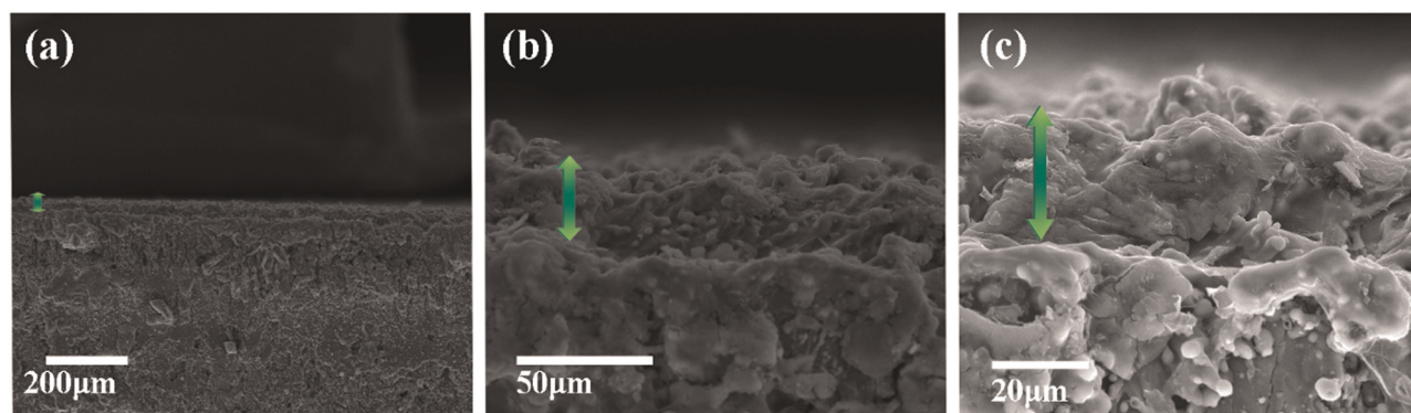
Figure S3: Cross-section FESEM image of S4 sample.
