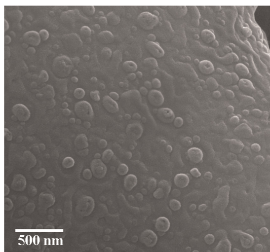
Figure S4: The SEM image of S4 through aging effect.
