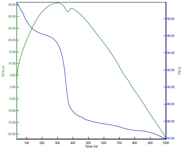
Figure S1: The TGA curve for MO2 ample.
