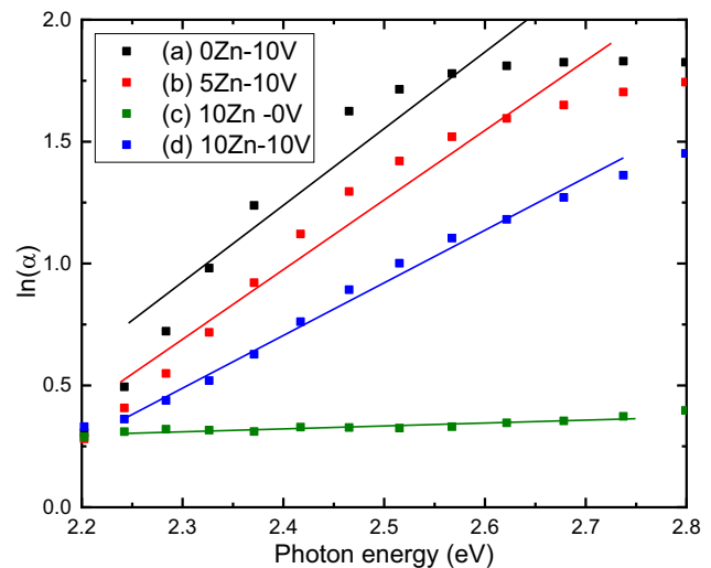
Figure 6: \ln(\alpha) vs photon energy of (a) V_2O_5 , (b) 5ZnO/10 V_2O_5 , (c) ZnO, and (d) 10ZnO/10 V_2O_5 nanocomposites.
