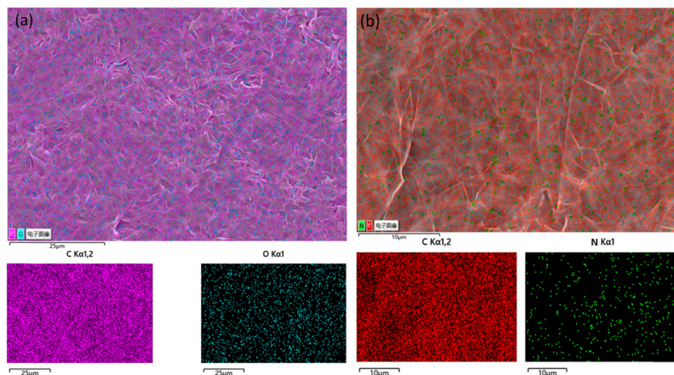
Figure S3: (a) STEM image and elemental mappings of the GUNS and (b) GUNS-N 2 .
