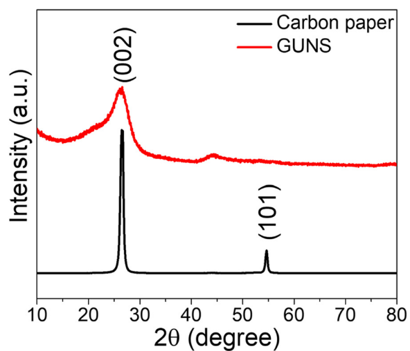
Figure S1: The XRD image of pristine carbon paper and GUNS.
