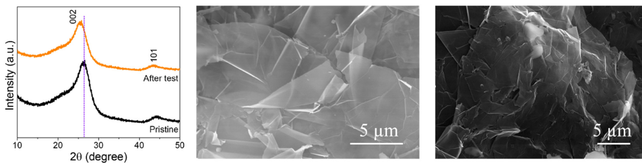
Figure S4: XRD and SEM results of pristine and after electrode test samples.
