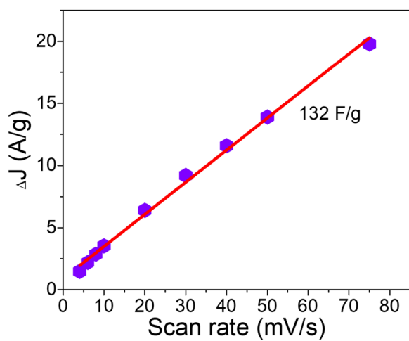
Figure S5: The C_{dl} value of GUNS.
