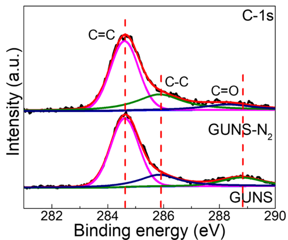
Figure S2: Deconvoluted XPS spectra of C-1s.
