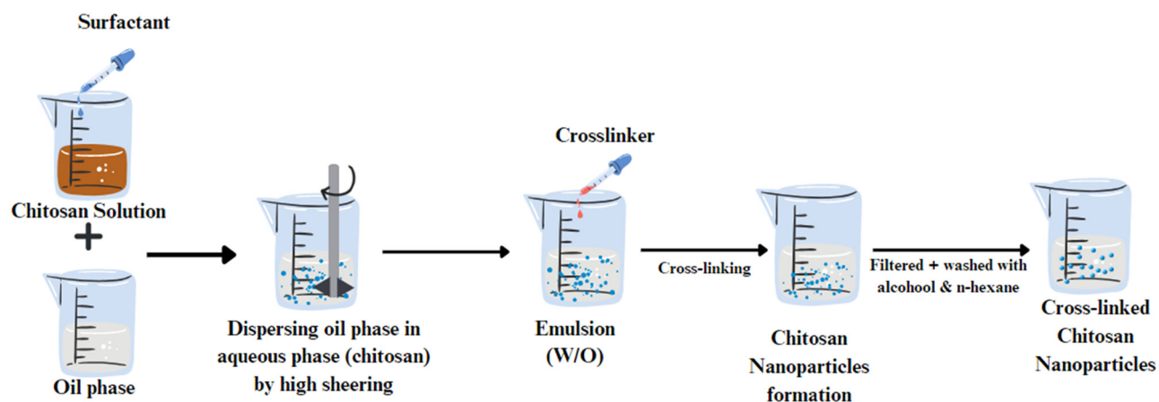
Figure 7: Schematic presentation of the emulsion crosslinking process.
