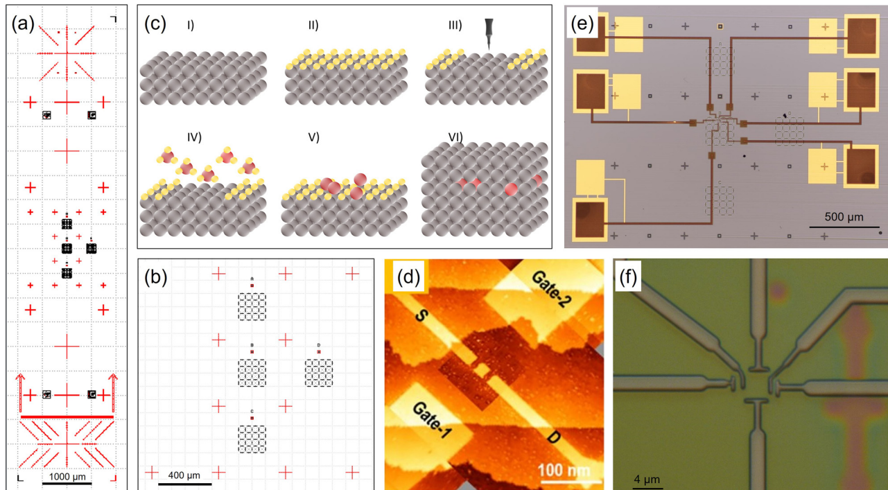
Figure 1: (a) Layout of registration marks on a chip showing the two sets of pre-patterned fiducial marks, namely the STM fiducial marks (the four black arrays of squares in the middle of the chip) and the global and local alignment marks for EBL (red marks). (b) Enlarged view of the array of squares used as STM fiducial marks on the center of the chip. (c) The main steps of hydrogen depassivation lithography for device fabrication: (I) clean silicon surface, (II) hydrogen passivation, (III) tip-induced lithography to selectively remove hydrogen atoms, phosphine (IV) dosing and (V) incorporation, and (VI) intrinsic silicon overgrowth. (d) STM images of a quantum dot connected to source and drain as well as two gate electrodes. (e) Large-scale optical image showing a finished chip with electrical leads from the device electrodes extending to bond pads. (f) Optical image of metal contacts over an encapsulated device.
