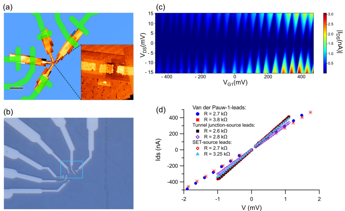
Figure 5: (a) STM image of a patterned SET with designed contacts (green) overlaid on the STM patterned contact pads; inset shows the core device region. (b) Contacts fabricated by EBL and subsequent metallization and anneal; the blue rectangle delimitates the region detailed in (a). (c) Transport measurements on the SET showing coulomb blockade oscillations demonstrating single electron tunneling events. (d) Two-point I–V plots from contact combinations on various devices.
