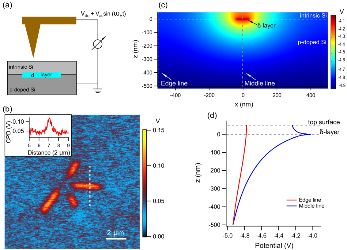
Figure 2: (a) KPFM setup over a Si-based heterostructure that incorporates a \delta -layer (blue) between the p-doped substrate (dark gray) and the nominally intrinsic top encapsulation (light gray). (b) KPFM contrast measured over an area consisting of a phosphorous-doped device. The inset shows tip-sample CPD along the dotted line. (c) The calculated 2D electrical potential map of a Si-based heterostructure that mimics the cross-section of the actual layer structure of a doped buried device. (d) Vertical cross-sections from (c) across regions with (middle line) and without (edge line) \delta -layer doping.
