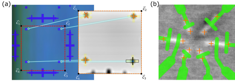
Figure 4: (a) Mapping an AFM topography (orange dashed outlined square in the middle of the figure) to the GDS-2 fiducial design coordinates (red dashed outlined square in the left part of the figure). The regions around the STM fiducial marks on the AFM topography (yellow rectangles) are analyzed to determine the centers of the fiducial marks (orange and black cross lines). Overlaid perpendicular (or near perpendicular) sampling regions (yellow rectangles) are chosen from the topography image to generate two center lines (orange solid lines) whose intersection defines the center of the circular etched feature; one bottom right sampling region is highlighted (black outline) and its corresponding center line is marked in black for clarity. The locations of these centers are then mapped (blue arrows) to the corresponding points on the GDS-2 file. (b) The final planned EBL contacts (green leads) are overlaid on the KPFM image (contact pads in white with ends marked by orange crosses).
