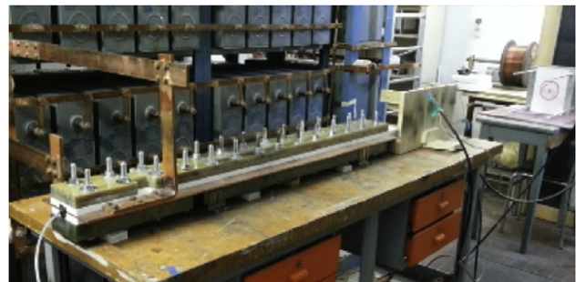
Figure 6: Railgun equipment setup [94].
