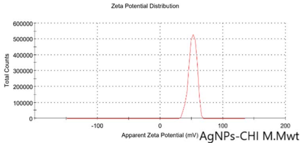
Figure S3: Zeta potential (mV) determined with a dynamic light scattering of the formulated silver nanoparticles reduced with medium molecular weight chitosan.
