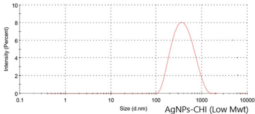
Figure S2: Dynamic light scattering of the formulated silver nanoparticles' mean size (nm) reduced with low molecular weight chitosan.
