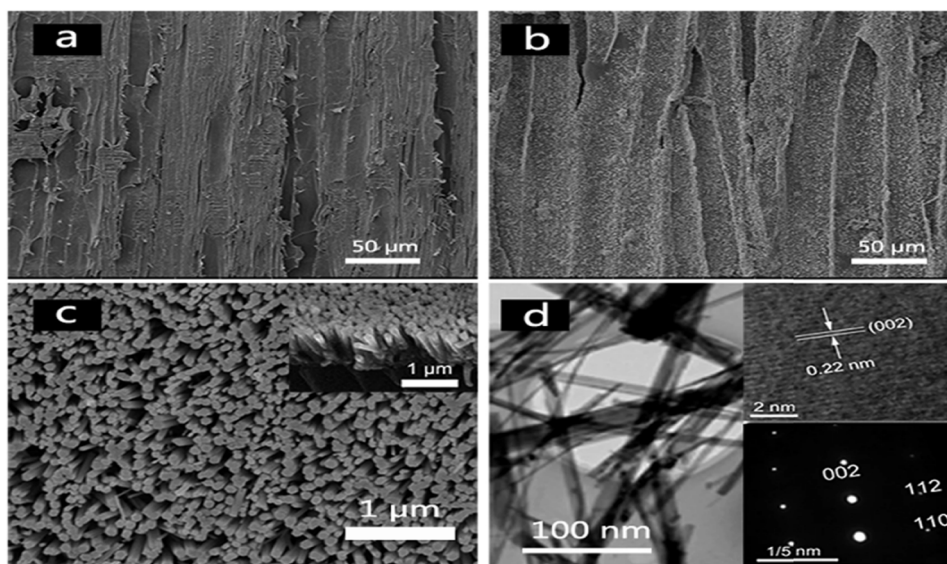
Figure 6: SEM image of the surface of (a) wood untreated, (b) wood with ZNAs in low magnification, (c) wood with ZNAs in high magnification, and (d) wood with ZNAs peeled off by the TEM image, HRTEM, and SAED pattern [90].
