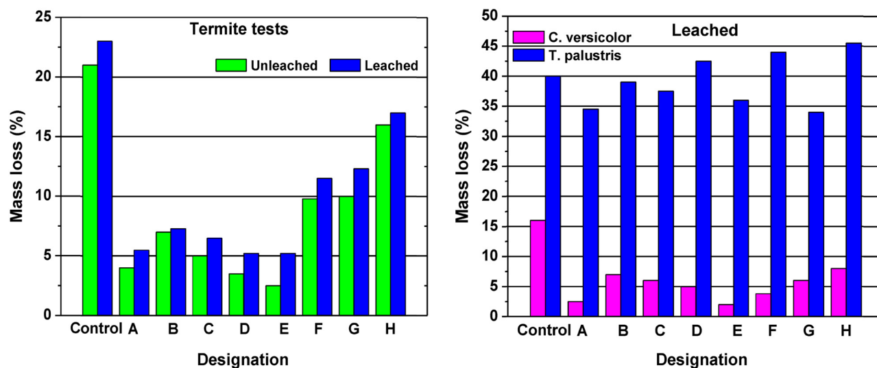
Figure 3: The mass loss (%) following termite resistance for leached and unleached pine wood: (i) nano-ZnO; (ii) nano-ZnO plus binder A; (iii) nano-ZnO plus binder B; (iv) nano-zinc borate; (v) nano-zinc borate plus binder A; (vi) nano-CuO; (vii) nano-CuO plus binder A; and (viii) nano-CuO plus binder B [71].
