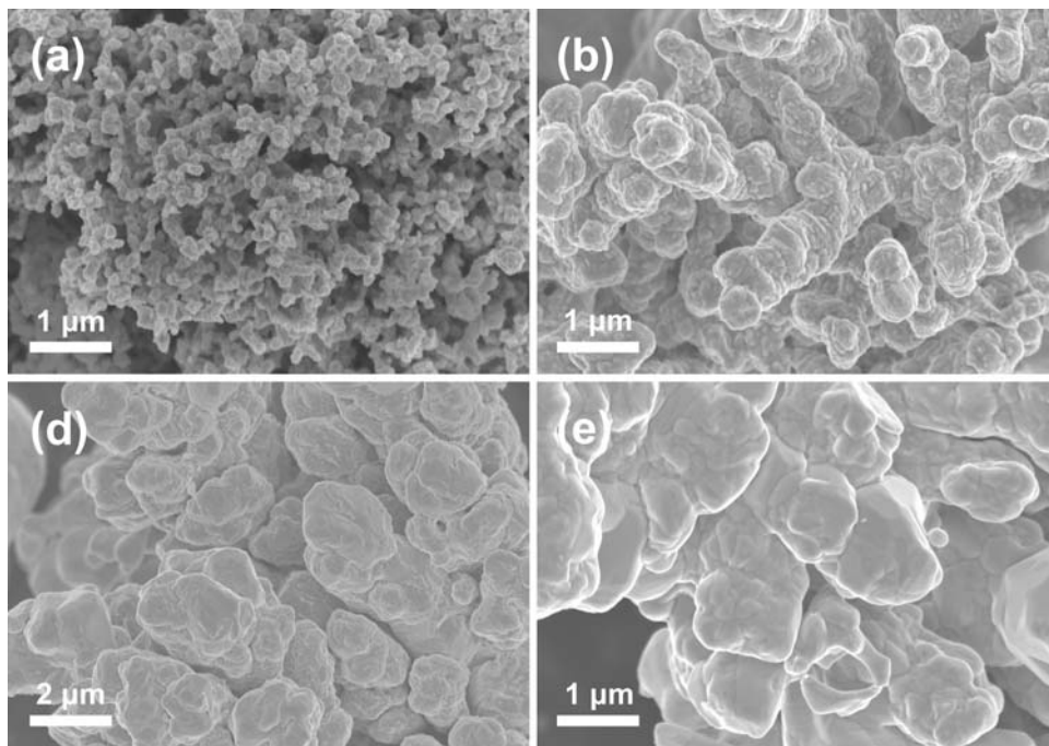
Figure S1: Figure S1: SEM images of copper particles with 0.1, 0.5, 2 and 5 μm in diameter.
