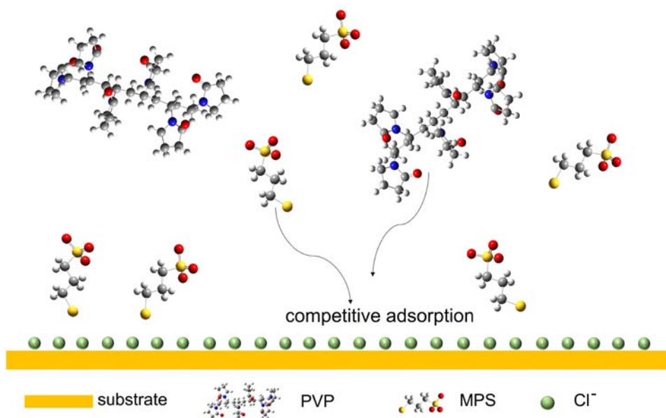
Figure S2: Schematic diagram of competitive adsorption in the solution with MPS and PVP. The cobalt electrodeposition was conducted in the bath and the cobalt pillar was fabricated in the solution with competitive adsorption of MPS and PVP. Chloride ions adsorb on the surface and accelerate the adsorption process of additives in the solution.
