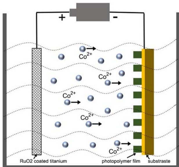
Figure S1: Schematic diagram of cobalt electrodeposition.
