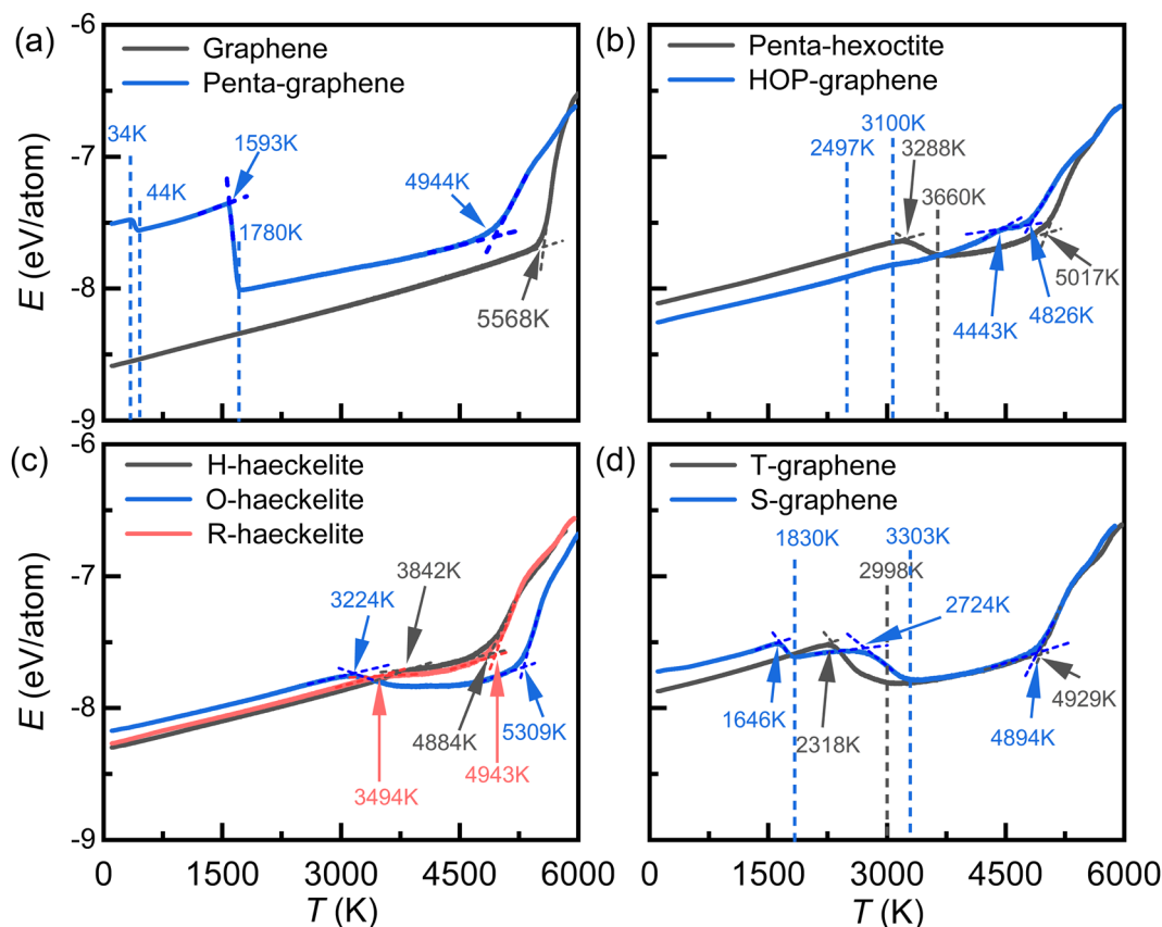
Figure 2: Variations in the potential energy ( E ) per atom with temperature for 2D carbon crystals of (a) graphene and penta-graphene; (b) penta-hexoctite and HOP-graphene; (c) H-, O-, and R-haekelites; and (d) T-graphene and S-graphene, respectively.
