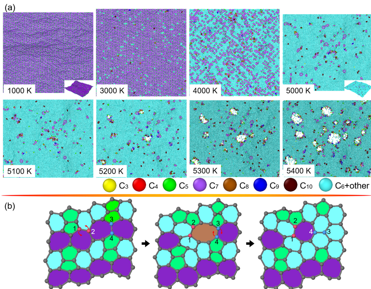
Figure 8: Structural changes in O-haekelite upon heating. (a) Top views of O-haekelite as the heating T increases from around 1,000 to 5,400 K. into melting phase. For eye-catching the thermally induced structural transformation in the O-haekelite, carbon atoms in polygonal rings from trigon to decagon are differently rendered. (b) Atomic illustration of nucleation of hexagons from pentagons, hexagons, and heptagons in a local region of O-haekelite. Particularly, some carbon atoms are number-ranked, and arrows are marked for revealing the origins of microstructural transitions.
