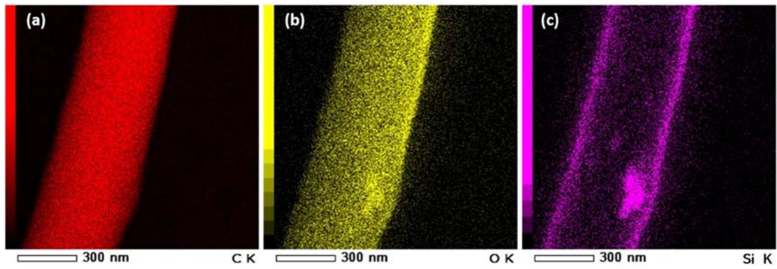
Figure S3: EDX mapping of ACNF incorporated with GRHC (GRHC/ACNF).
